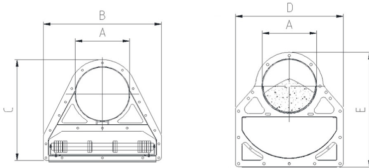
Image: Roller-carried return (RCR) and Air-carried return (ACR)
