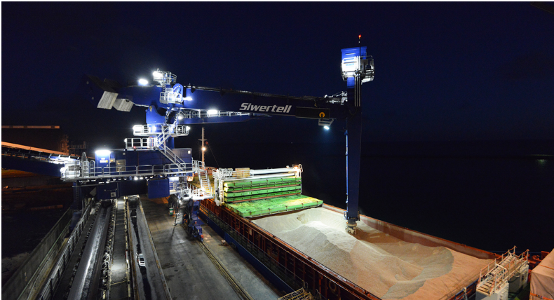
SIWERTELL SHIP UNLOADER - DENMARK
