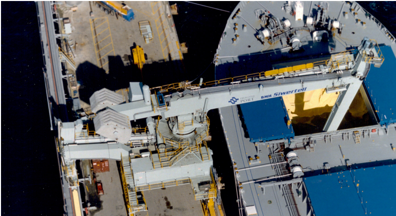
SIWERTELL SHIP UNLOADER - AUSTRALIA
